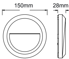
SLIM02*
