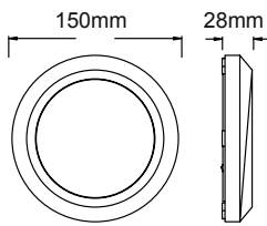
SLIM01*
