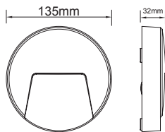
SLIM41*
