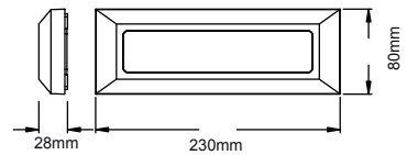
SLIM31*
