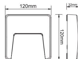
SLIM42*
